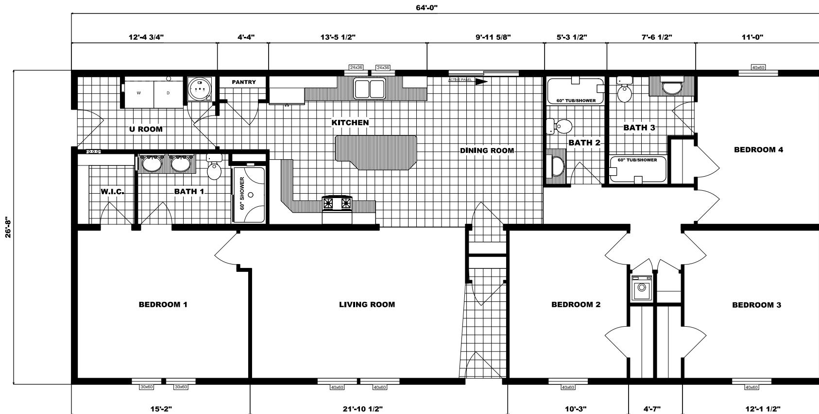
FLOOR PLAN NETR G-3604 26'8" X 64' FOUR BEDROOM, THREE BATH APPROX. 1706 SQ. FT.
