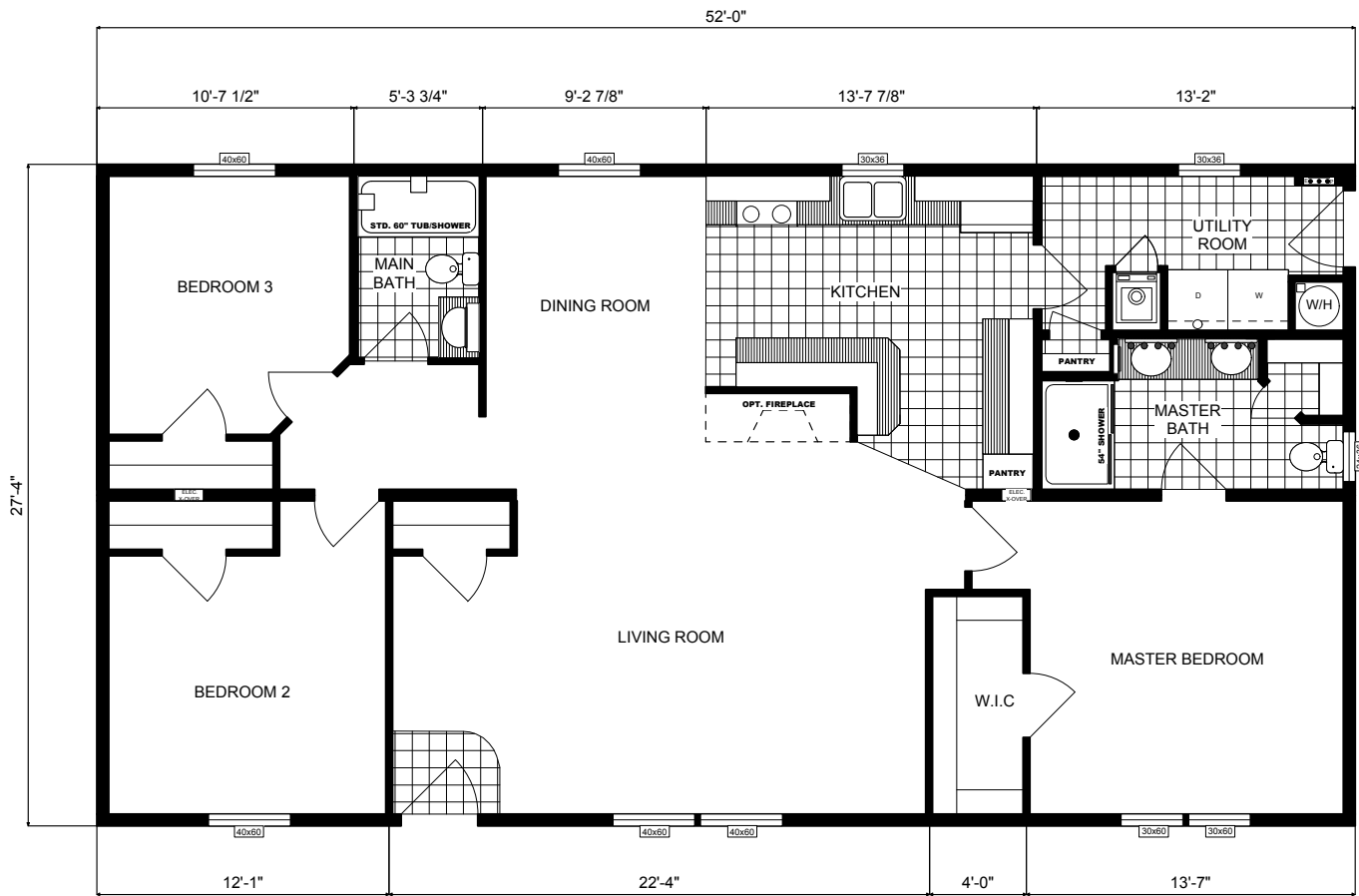
FLOOR PLAN GH-1772 28X52 THREE BEDROOM, TWO BATH APPROX. 1421 SQ. FT.
