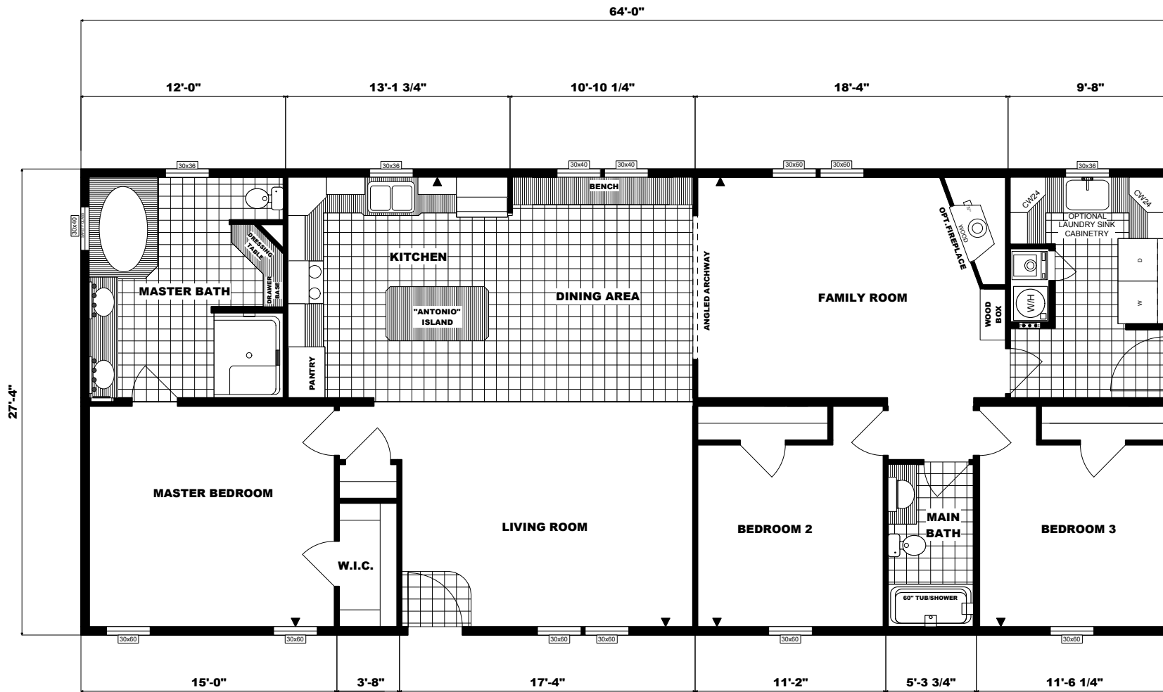
FLOOR PLAN G3653 28X64 THREE BEDROOM, TWO BATHS APPROX. 1749 SQ. FT.
