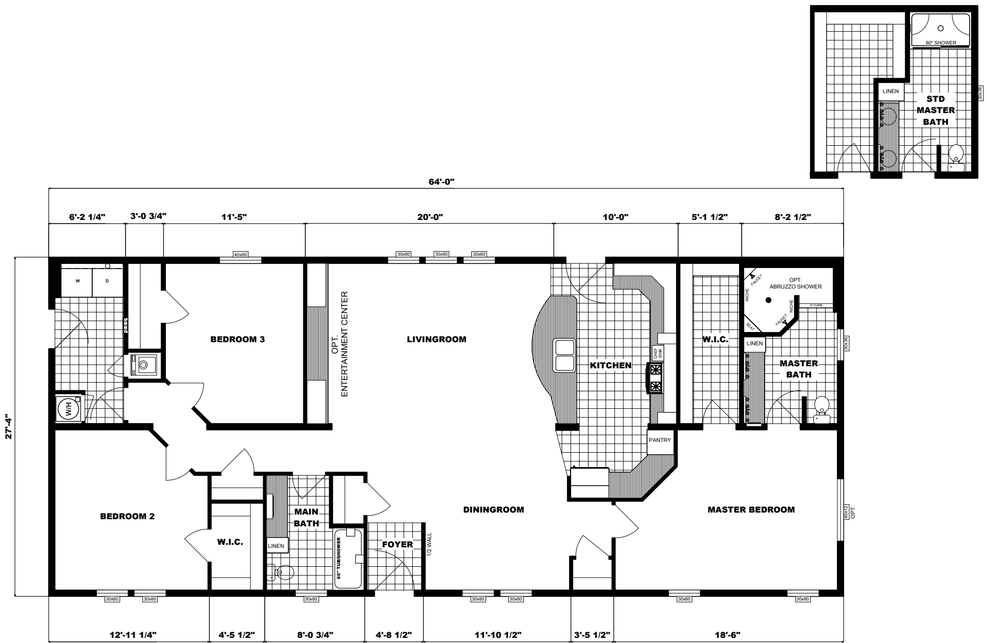
FLOOR PLAN G3647 28X54 THREE BEDROOM, TWO BATH APPROX. 1749 SQ. FT.
