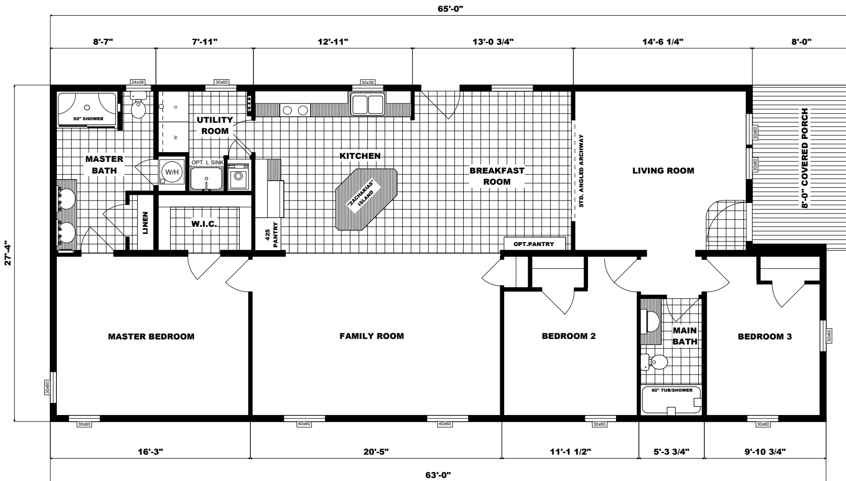
FLOOR PLAN G 3602 28X65/63 W/8'-0" COVERED PORCH FAMILY ROOM THREE BEDROOM, TWO BATH APPROX. 1646 SQ. FT.
