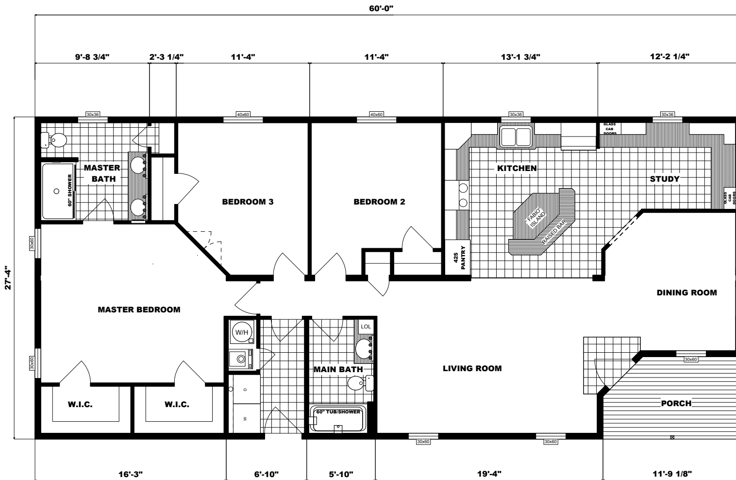
FLOOR PLAN G-3556 28X60 THREE BEDROOM, TWO BATH APPROX. 1564 SQ. FT.
