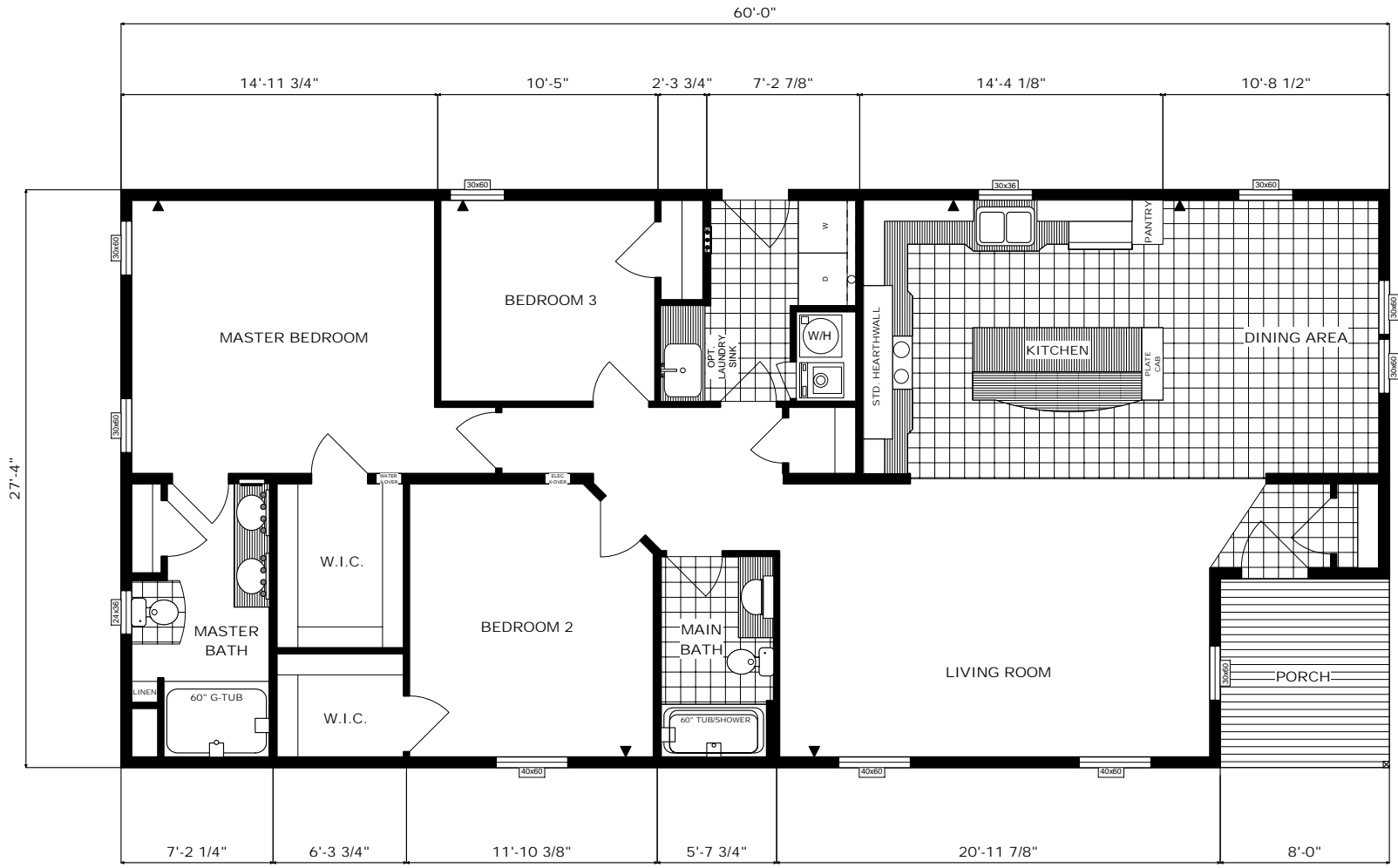
FLOOR PLAN G-3552 28X60 THREE BEDROOM, TWO BATH HEARTH KITCHEN AND COVERED PORCH APPROX. 1422 SQ. FT.
