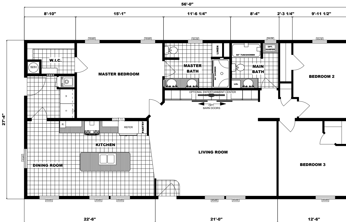
FLOOR PLAN G3462 28X56 THREE BEDROOM, TWO BATH APPROX. 1531 SQ. FT.
