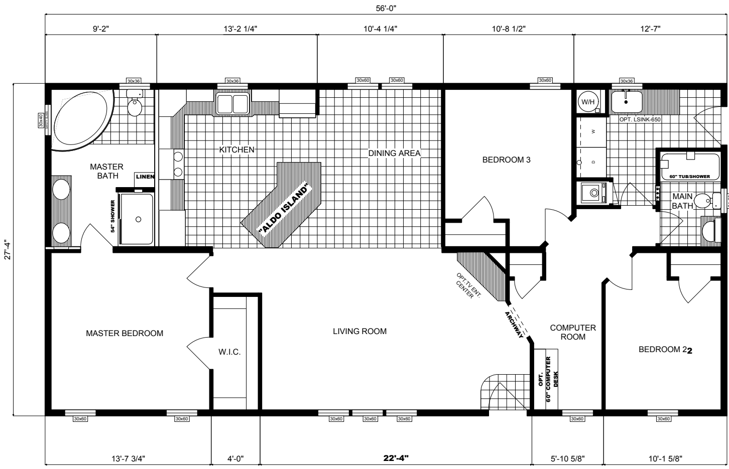
FLOOR PLAN G3450 28X56 THREE BEDROOM, TWO BATHS NAPOLI FIRESIDE HEARTH APPROX. 1531 SQ. FT.
