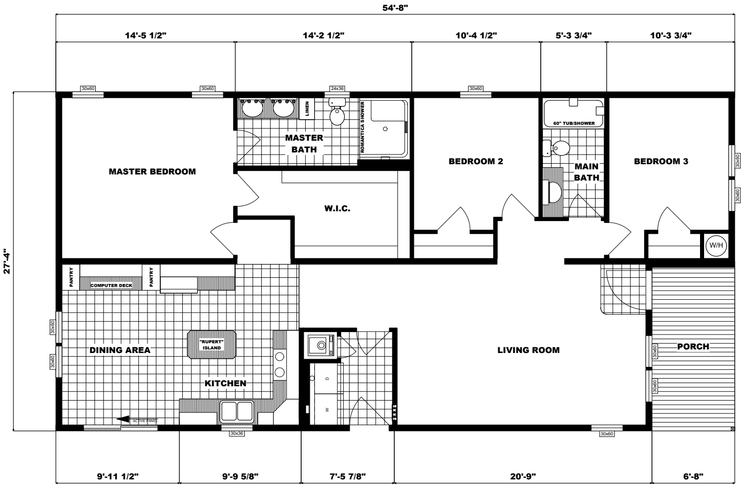
FLOOR PLAN G-3400 28X54'8" THREE BEDROOM, TWO BATH APPROX. 1406 SQ. FT.
