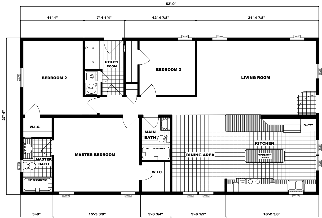
FLOOR PLAN G-3358 28X52 THREE BEDROOM, TWO BATH APPROX. 1422 SQ. FT.
