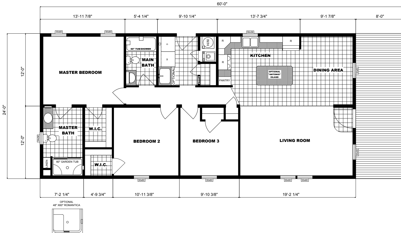
FLOOR PLAN G-294 28X52 W/ 8'0" PORCH THREE BEDROOM, 2 BATH APPROX. 1248 SQ. FT.
