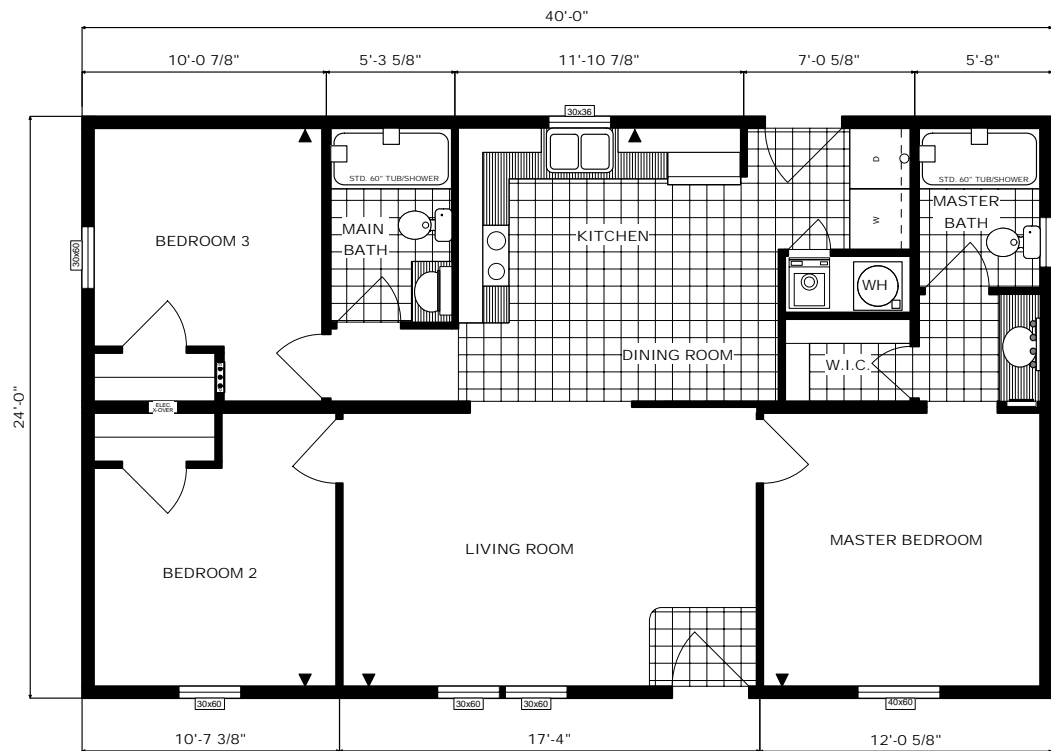
FLOOR PLAN G-200 24X40 THREE BEDROOMS, TWO BATHS APPROX. 960 SQ. FT.
