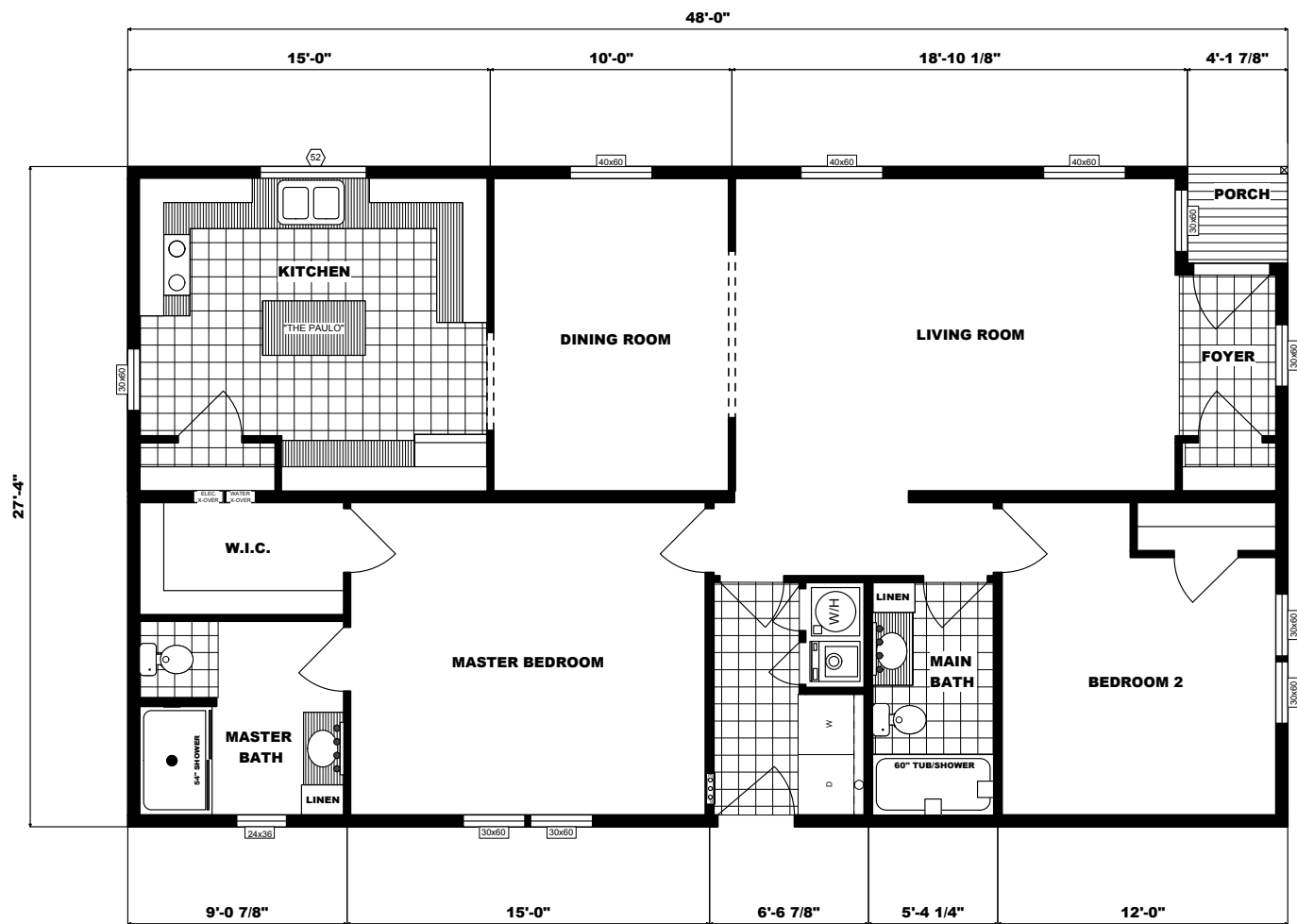
FLOOR PLAN G1870 28X48 TWO BEDROOM, TWO BATH APPROX. 1313 SQ. FT.
