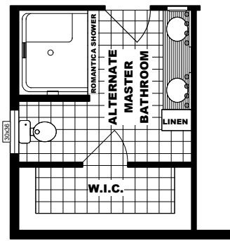
FLOOR PLAN G-1836 28X60 THREE BEDROOM, TWO BATH APPROX. 1534 SQ. FT.
