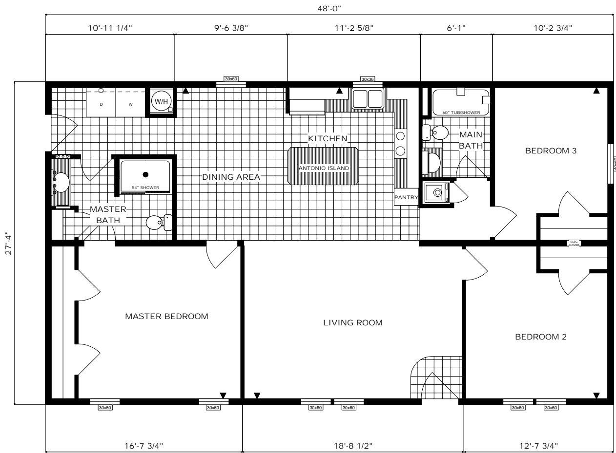
FLOOR PLAN G-1753 28X48 3 BEDROOM, 2 BATHS APPROX. 1312 SQ. FT.
