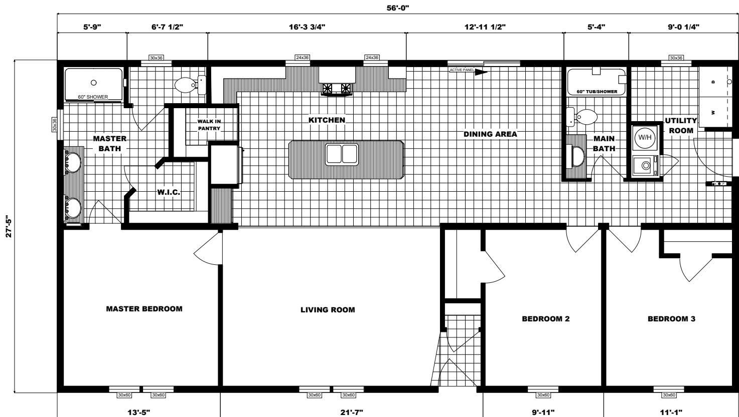
FLOOR PLAN G3465 28X56 THREE BEDROOM, TWO BATH APPROX.1533 SQ. FT.
