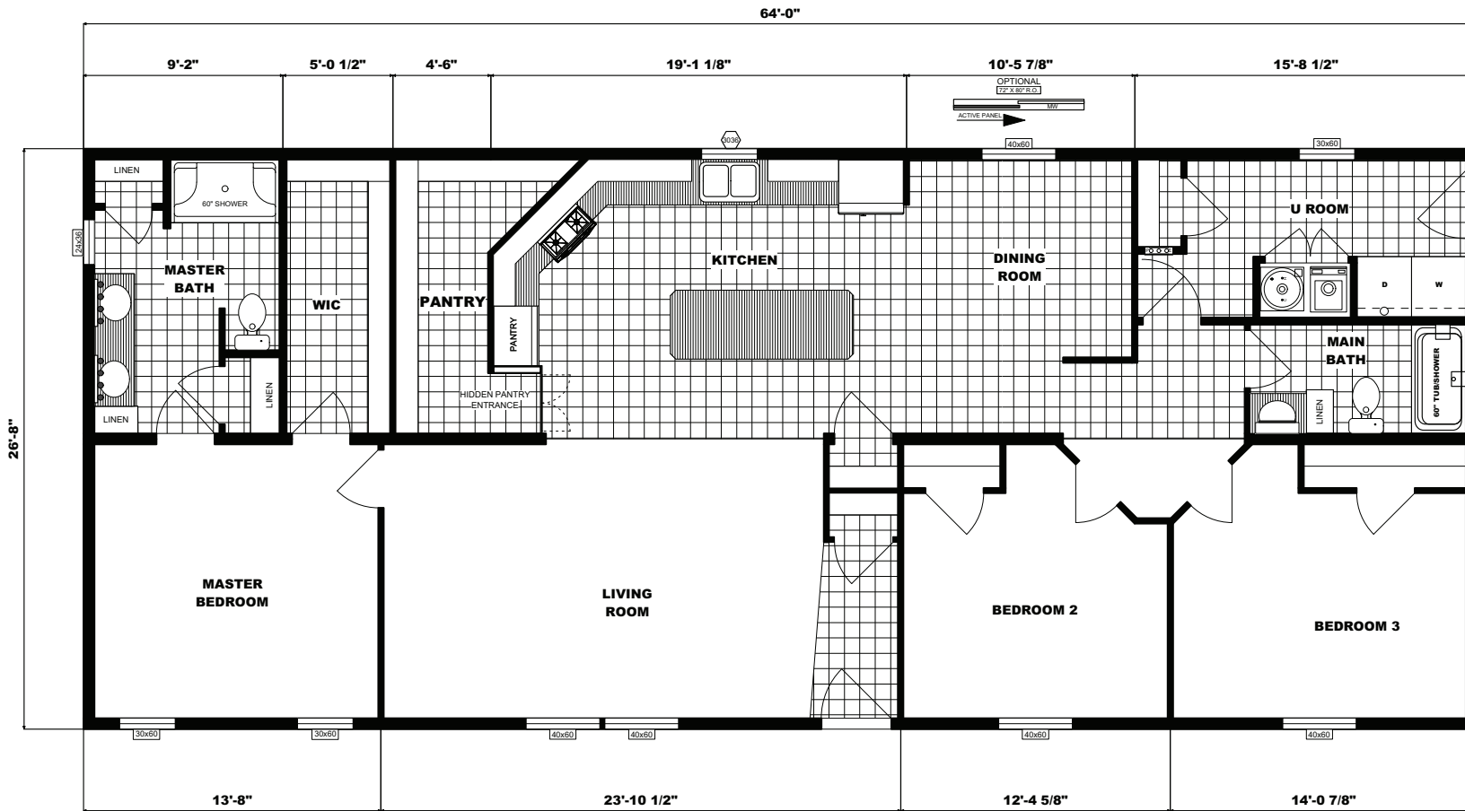
FLOOR PLAN NETR-G-3644 26'8"X64 THREE BEDROOM, TWO BATH APPROX. 1706 SQ. FT.
