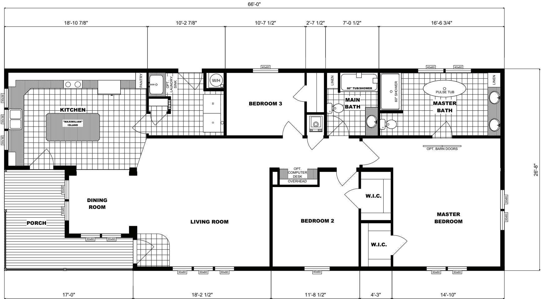
FLOOR PLAN NETR-G3655 26'8"X66' THREE BEDROOM, TWO BATH APPROX. 1614 SQ. FT. WITH 146 SQ.FT. PORCH
