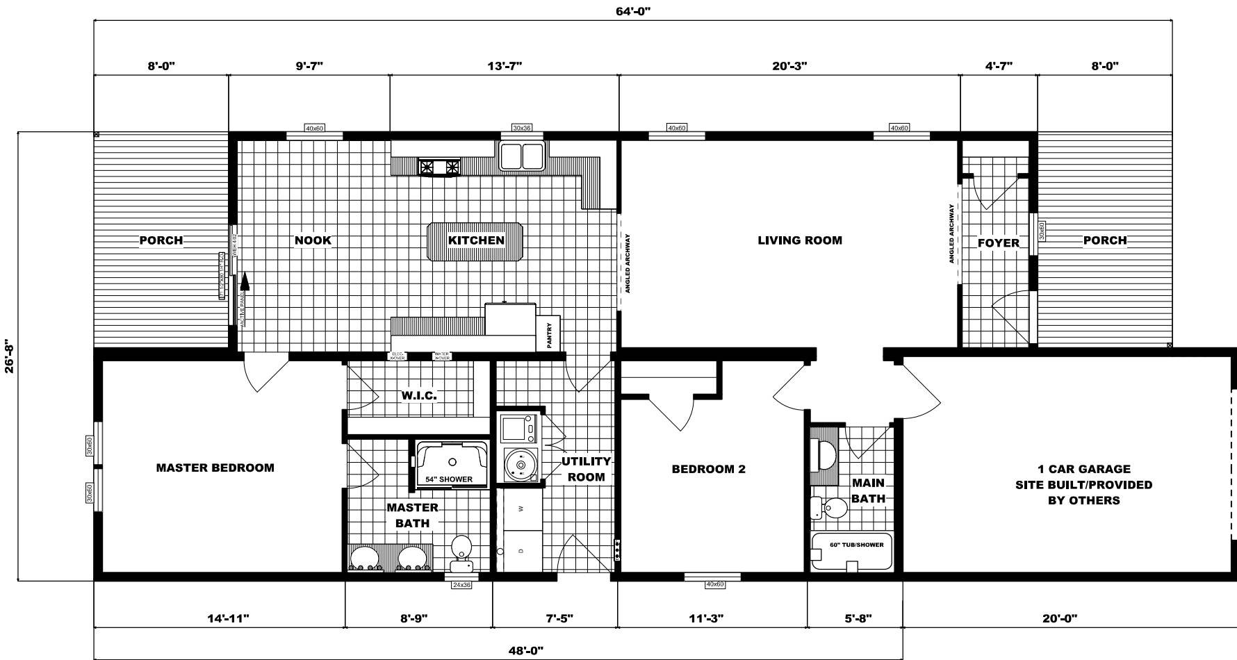
FLOOR PLAN NETR-G1815 28X64/48 TWO BEDROOM, TWO BATH APPROX. 1488 SQ. FT.
