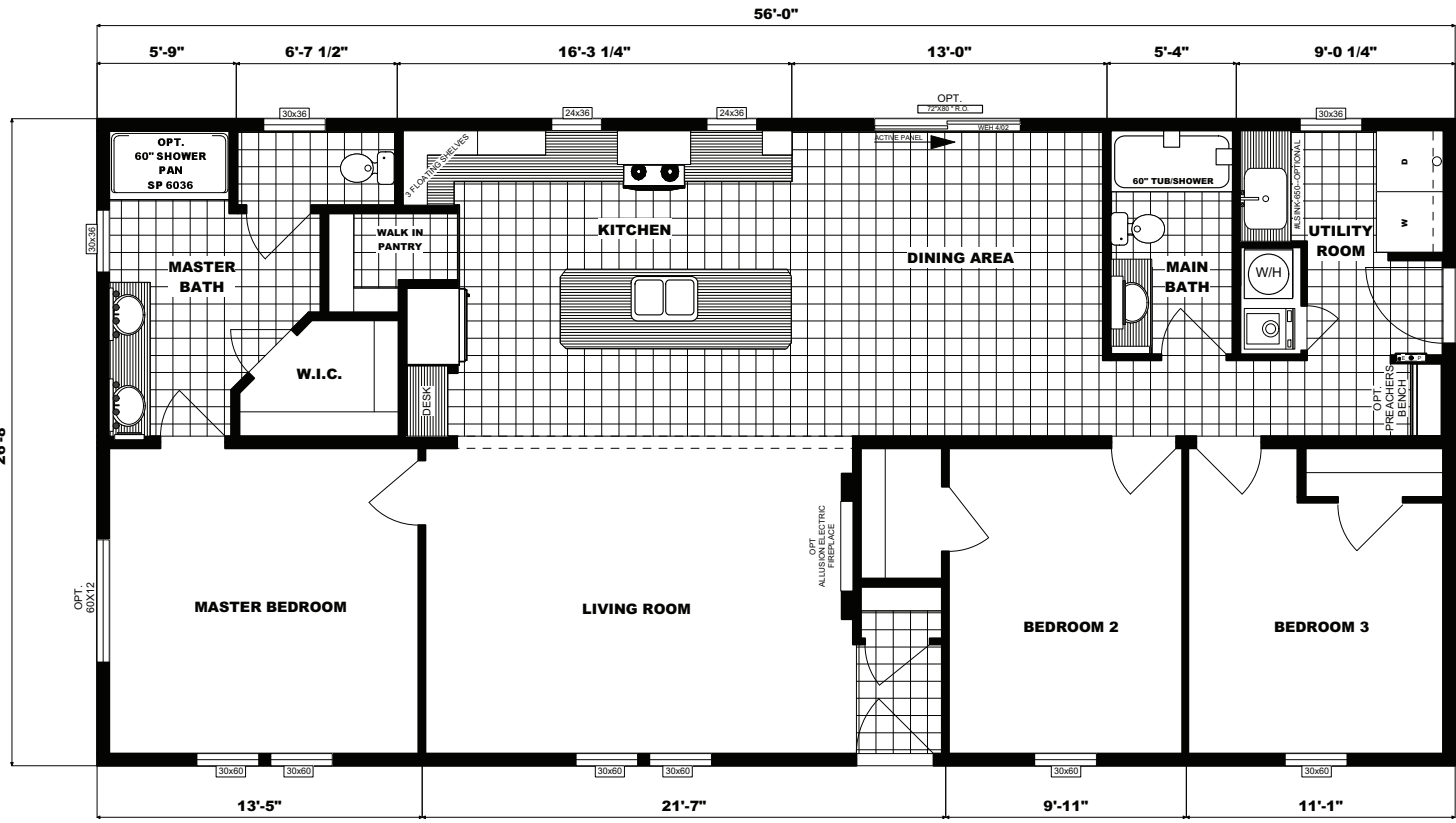
FLOOR PLAN NETR 3465 28X56 THREE BEDROOM, TWO BATH APPROX.1493 SQ. FT.
