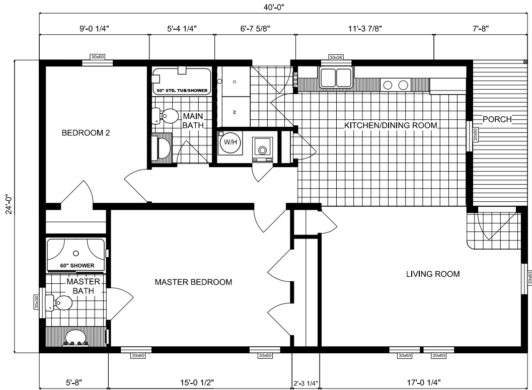
FLOOR PLAN GH-203 24X40 TWO BEDROOM, TWO BATH APPROX. 960 SQ. FT.
