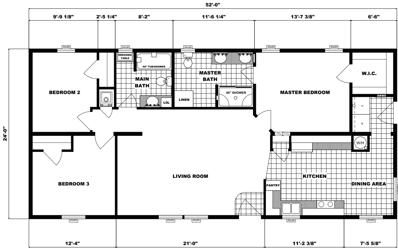
FLOOR PLAN GH-230 24X48 THREE BEDROOM, TWO BATH APPROX. 1248 SQ. FT.
