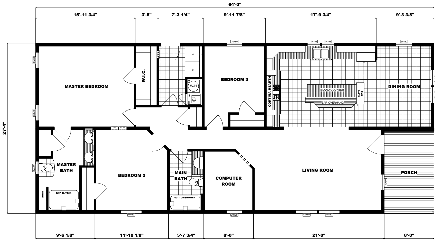
FLOOR PLAN GH-1880 28X64 THREE BEDROOM, TWO BATH CORTINA HEARTH KITCHEN APPROX. 1749 SQ. FT.
