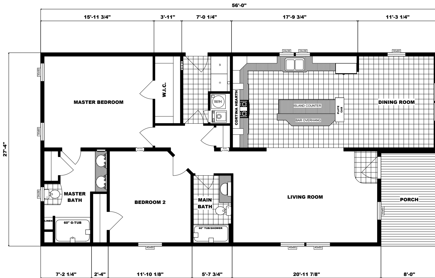
FLOOR PLAN GH-1860 28X56 TWO BEDROOM, TWO BATH CORTINA HEARTH KITCHEN AND COVERED PORCH APPROX. 1422 SQ. FT.
