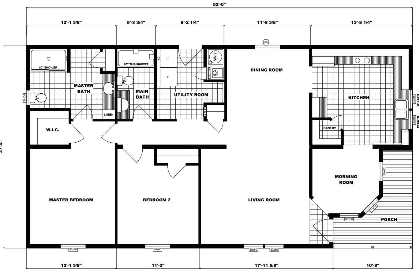
FLOOR PLAN GH1723 28X52 TWO BEDROOM, TWO BATH APPROX. 1334 SQ. FT.
