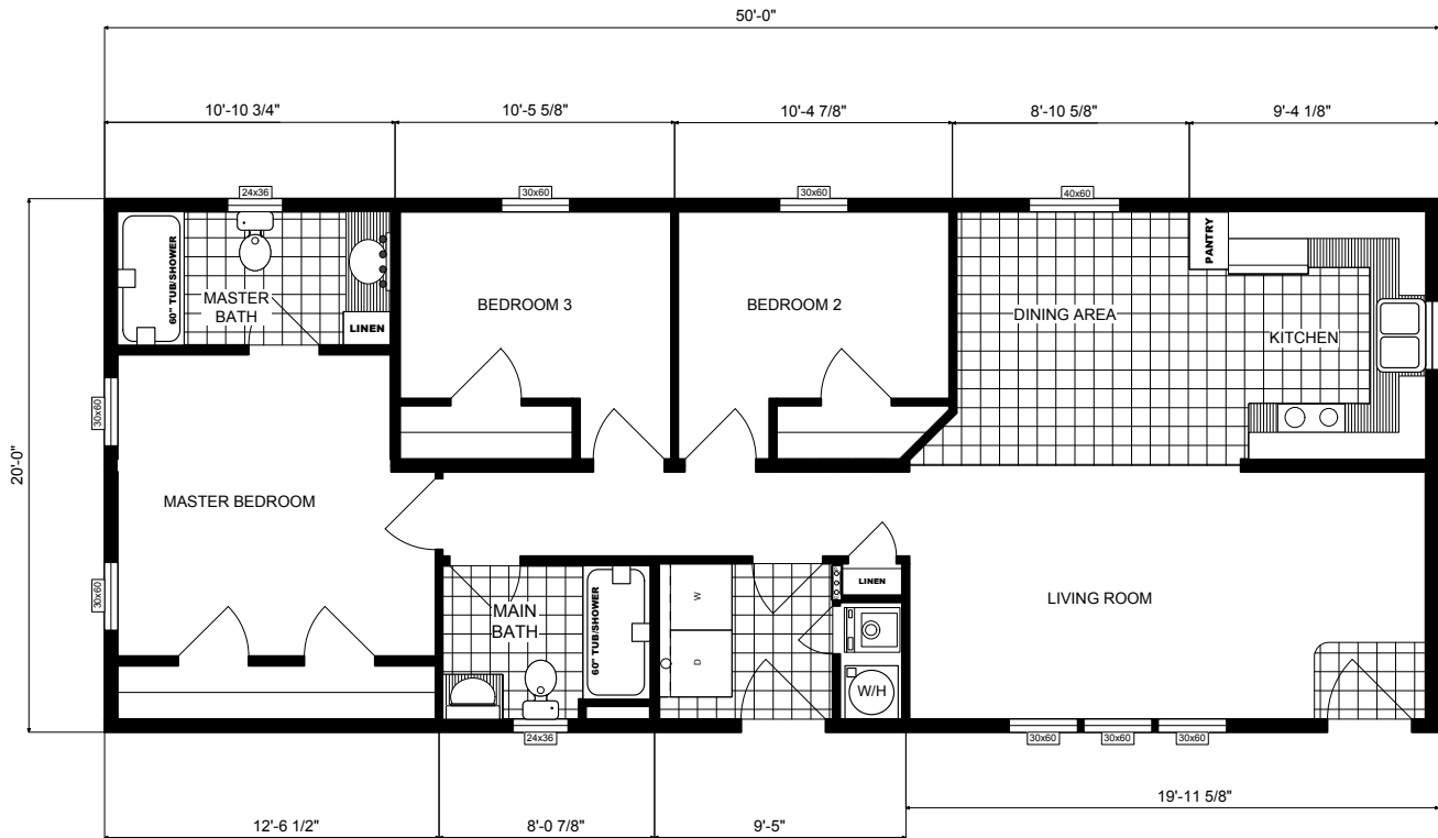
FLOOR PLAN GH136 20X50 THREE BEDROOM TWO BATH APPROX. 972 SQ. FT.
