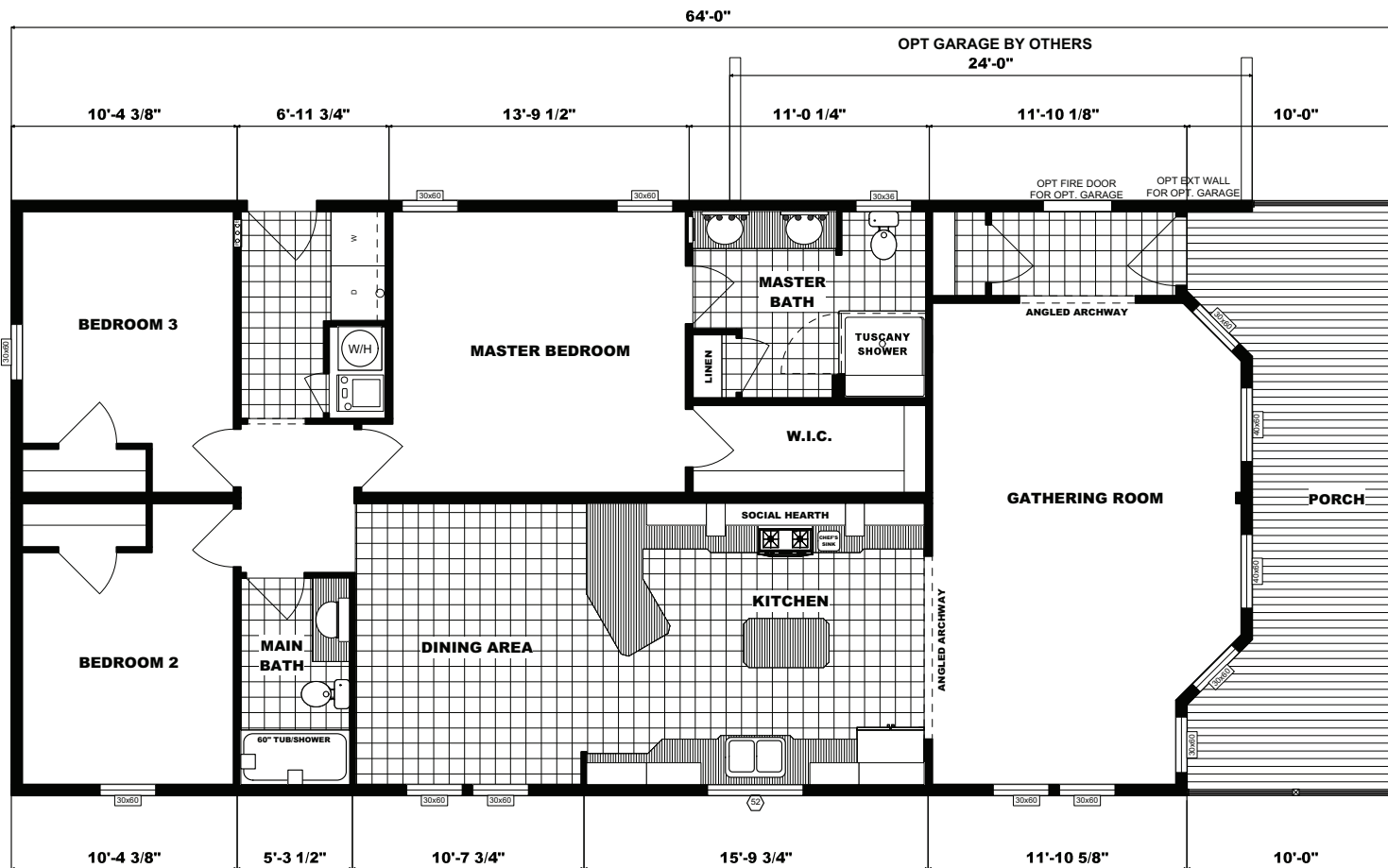
FLOOR PLAN G-3645 28X64 THREE BEDROOM, TWO BATH APPROX. 1524 SQ. FT.
