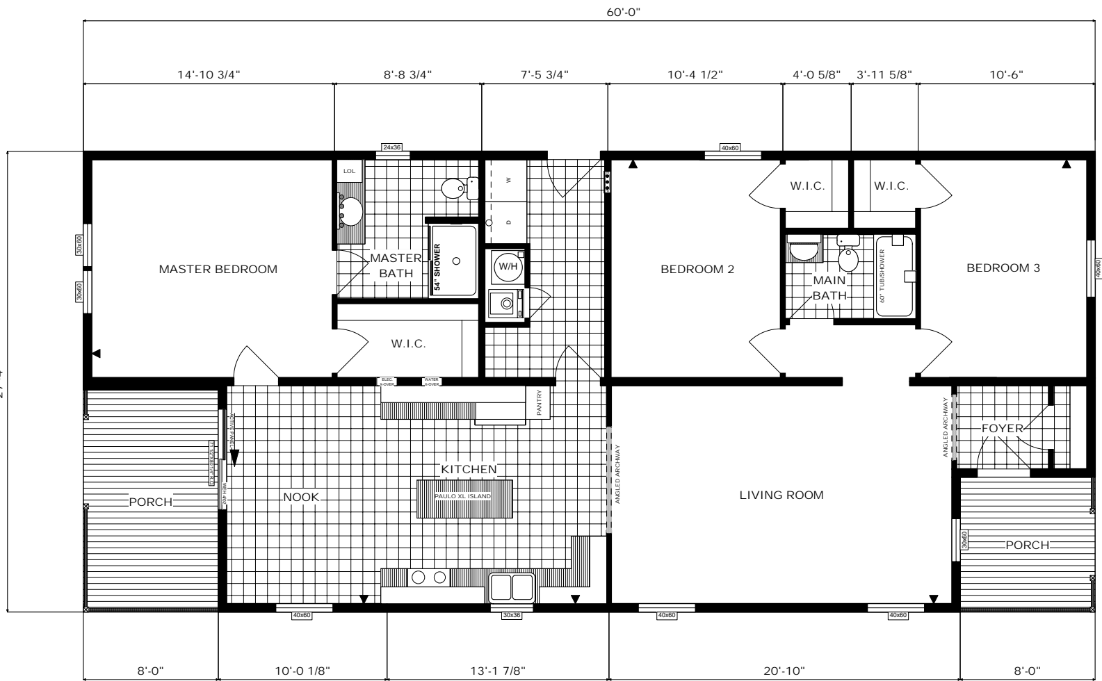
FLOOR PLAN G-3551 28X60 THREE BEDROOM, TWO BATH APPROX. 1470 SQ. FT.
