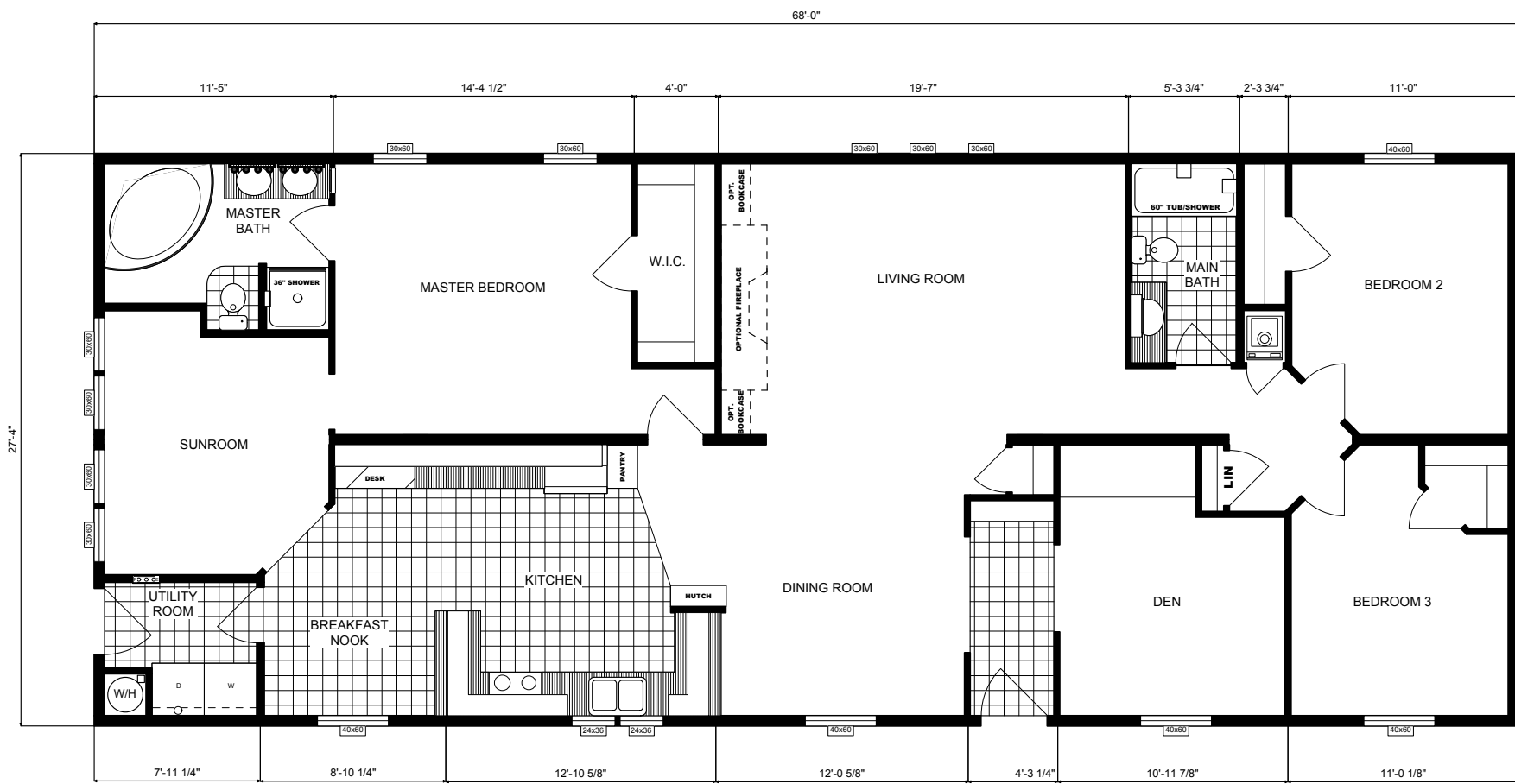
FLOOR PLAN G-2053 28X68 THREE BEDROOM, TWO BATH DEN AND SUNROOM APPROX. 1858 SQ. FT.
