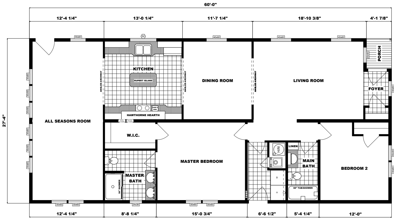
FLOOR PLAN G 1873 28X60 ALL SEASON ROOM TWO BEDROOM, TWO BATH APPROX. 1640 SQ. FT.
